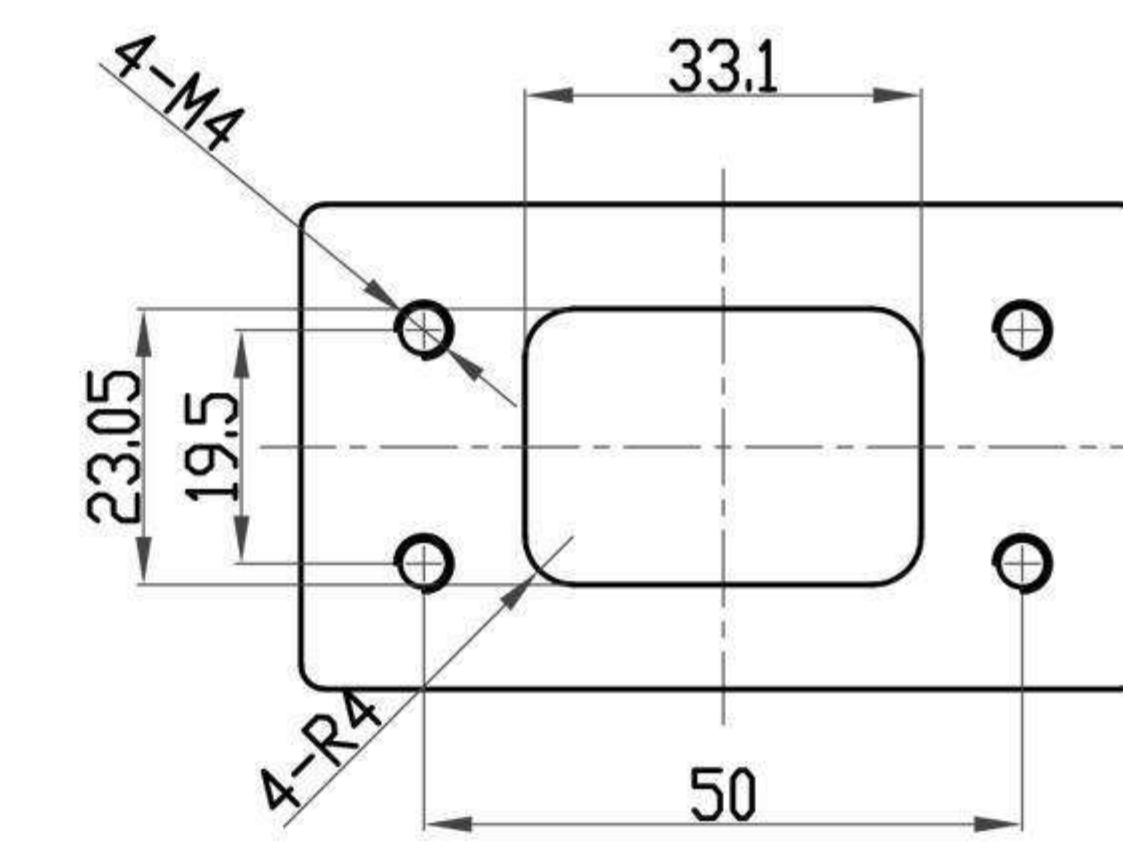
Socket mounting panel T=3.0mm Panel tolerance: \pm 0.05
