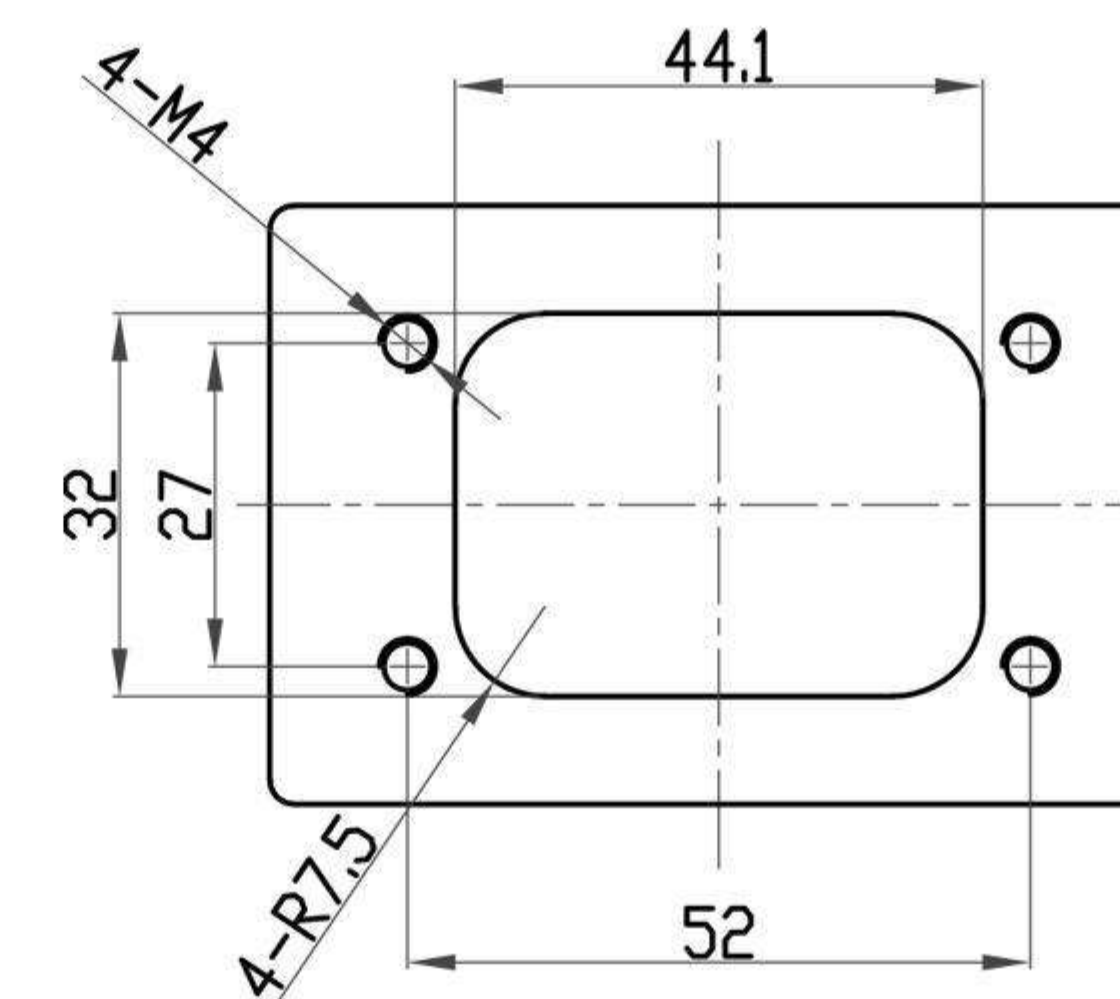
Plug mounting panel T=3.0mm Panel tolerance: \pm 0.05
